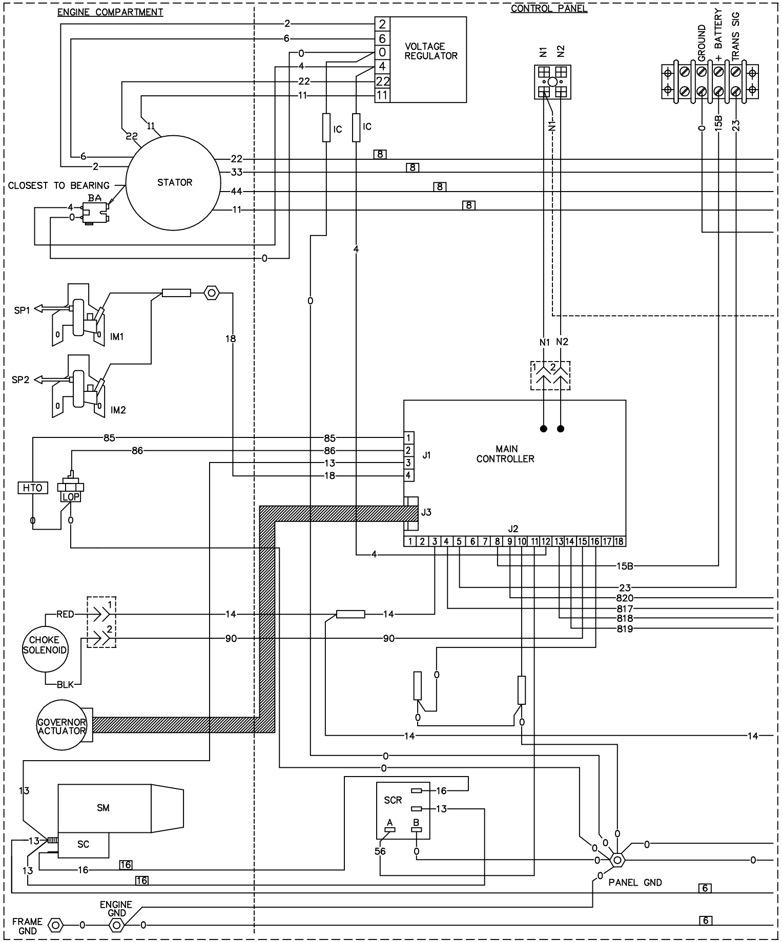
WIRING - DIAGRAM 2008 AIR COOLED DRAWING #: 0G8186
