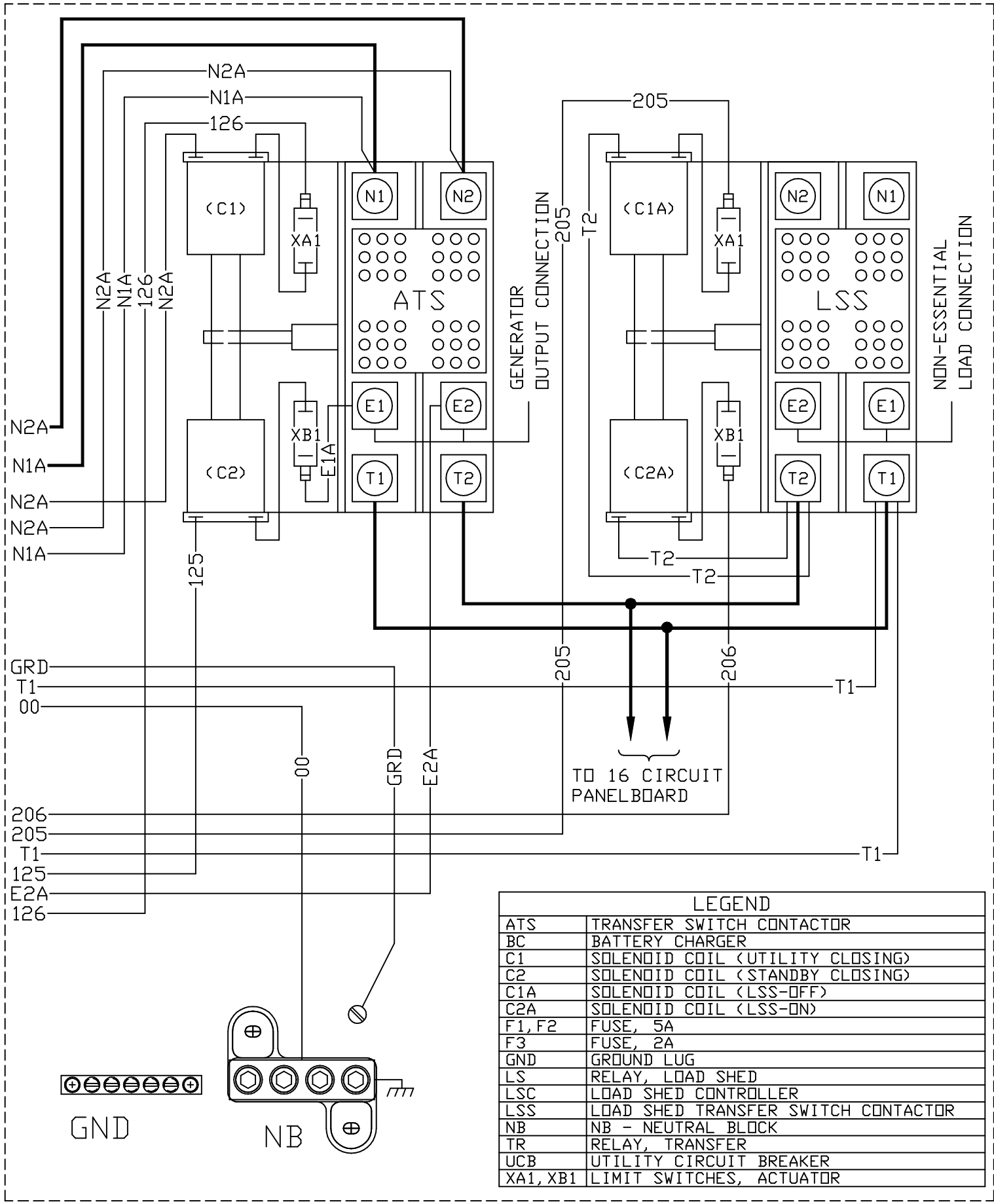
WIRING - DIAGRAM LOAD SHED SWITCH DRAWING #: 0G7817
